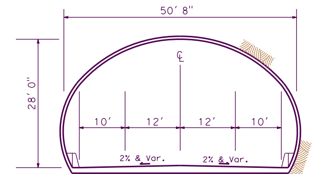
Typical Tunnel
